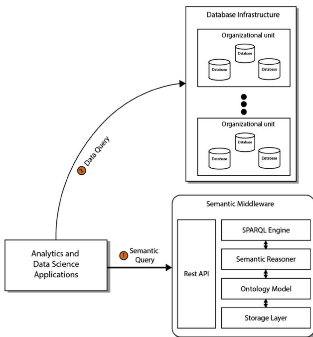
Figure 2 – MINDSense: a semantic middleware for industrial sensors
